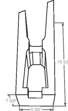
6x8x16 22.5 DEGREE MITER
