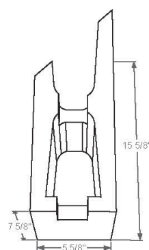
6x8x16 45 DEGREE MITER
