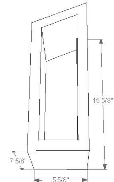
6x8x16 22.5 DEGREE MITER SINGLE CORE
