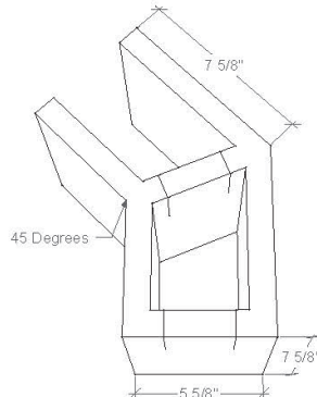
6x8x16 CHEVRON
