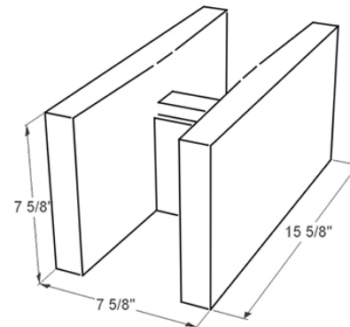
DOUBLE OPEN END BOND BEAM
