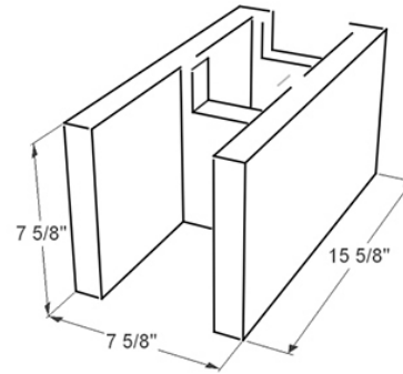
SINGLE OPEN END BOND BEAM
