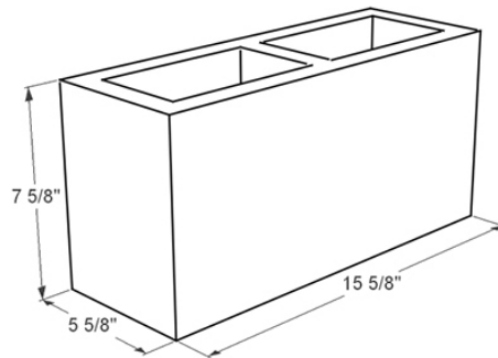
STANDARD (6 IN WIDTH)
