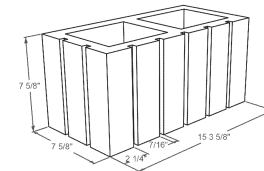
8x8x16 505 Score 1 Side 1 End
