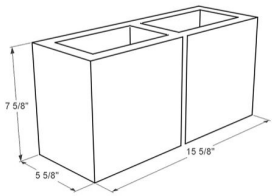
6x8x16 Vertical Score
