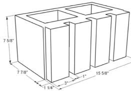
8x8x16 301 Score 1 Side
