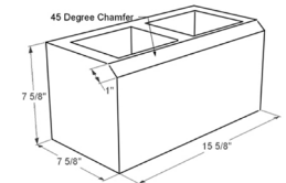
8x8x16 With 1 Inch Chamfer
