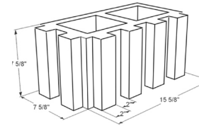
8x8x16 202 Score 1 Side 1 End
