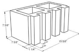
8x8x16 202 Score 1 Side
