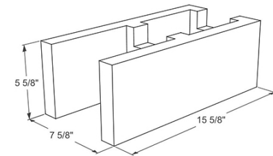
OPEN END BOND BEAM (8x6x16)
