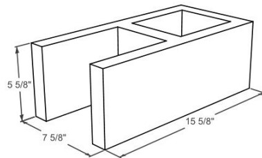
OPEN END (8x6x16)
