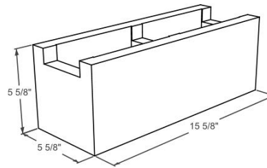
BOND BEAM (6x6x16)
